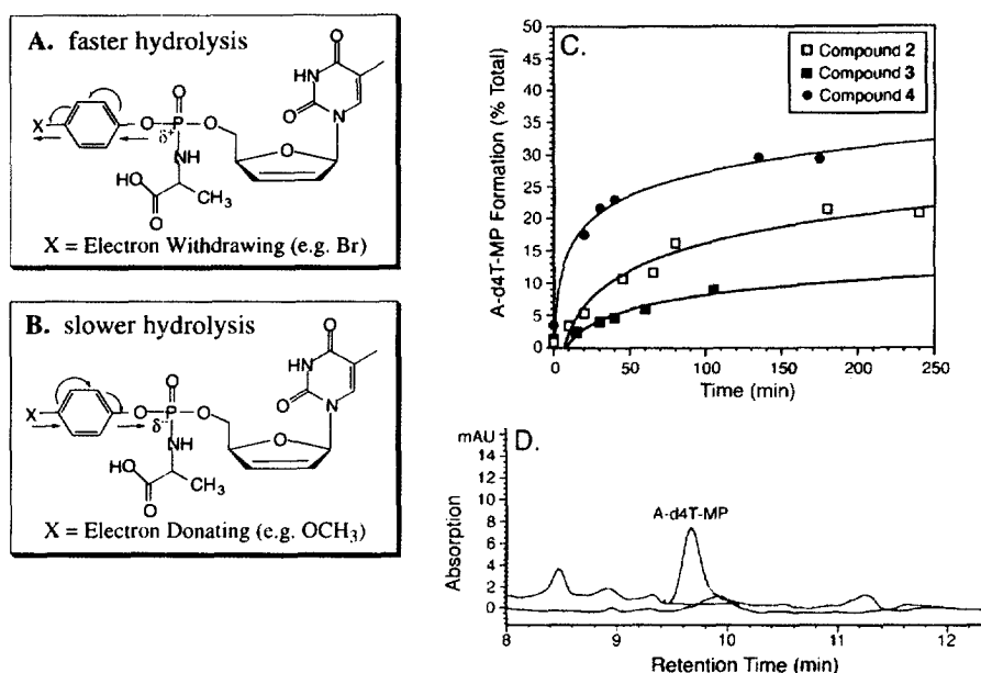
Figure 2. Susceptibility of compounds 2–4 to hydrolysis. (A and B) Schematic representation of the electronic effects of the para substituent in the phenyl ring of metabolite precursor B (see Fig. 1). (C) Compounds 2–4 were dissolved in methanol and then treated with 0.002 N NaOH. The concentrations were kept constant and the generation of the hydrolysis product A-d4T-MP was monitored using HPLC. A Lichrospher column (C18) was used for the HPLC runs. The column was eluted under isocratic conditions using the solvent mixture 70/30 water/acetonitrile. (D) Compounds 2 and 4 (1 mM in Tris-HCl) were incubated with 100 U of porcine liver esterase (Sigma) in Tris-HCl buffer (pH 7.4) for 2 h at 37 °C. Reaction was stopped by adding acetone and chilling the reaction mixture. Following centrifugation at 15,000 × g, 0.1 mL aliquots of the reaction mixture were examined for the presence of the active metabolite A-d4T-MP by using a quantitative analytical HPLC method capable of detecting 50 pmols of the metabolite. The 0.1 mL aliquot of the reaction product of compound 4 contained 1.4 nmols of A-d4T-MP , whereas no metabolite was detected in the reaction product of compound 2.
