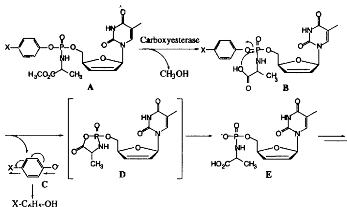
Figure 1. Literature proposed metabolic pathway of aryl phosphate derivatives of d4T. 8
